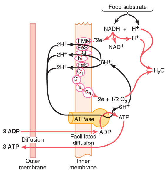
Figure 68-7. Mitochondrial chemiosmotic mechanism of oxidative phosphorylation for forming large quantities of ATP. This figure shows the relationship of the oxidative and phosphorylation steps at the outer and inner membranes of the mitochondrion. FeS, iron sulfide protein; FMN, flavin mononucleotide; Q, ubiquinone.
