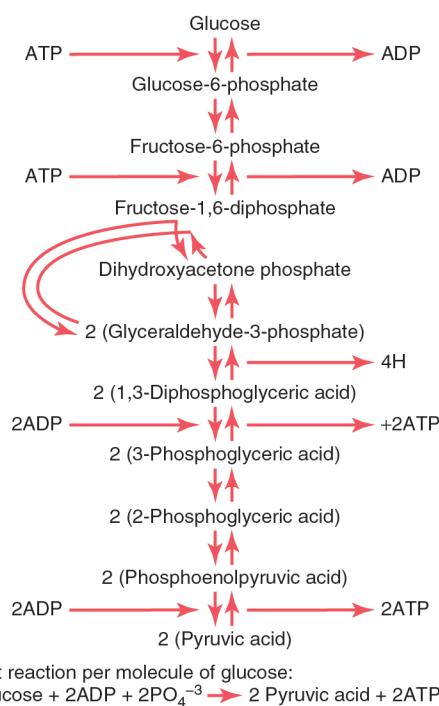
Figure 68-5. Sequence of chemical reactions responsible for glycolysis.
