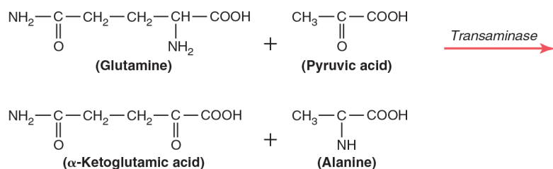
Figure 70-3. Synthesis of alanine from pyruvic acid by transamination.
